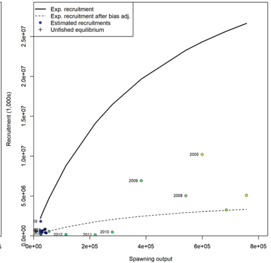
Figure A.1. Stock-recruit curves for the modeling-based alternative models (2025.2-5a). Each stock-recruit curve shows the mean expected recruitment (solid curve), expected recruitment after bias adjustment (dashed line), and annual stock-recruit data (labeled points).
