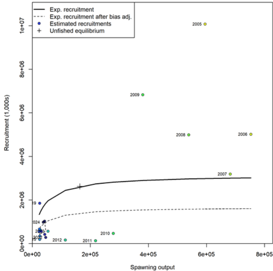
Figure A.1. Stock-recruit curves for the modeling-based alternative models (2025.2-5a). Each stock-recruit curve shows the mean expected recruitment (solid curve), expected recruitment after bias adjustment (dashed line), and annual stock-recruit data (labeled points).
