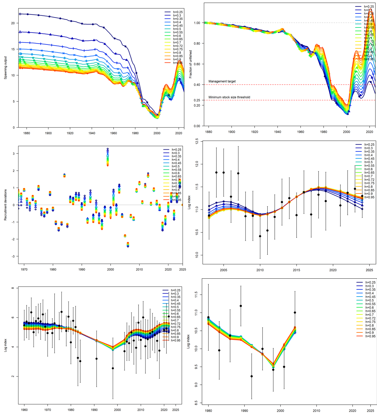
Figure 17D. Likelihood profiles for the Beverton-Holt steepness parameter ( h ). Spawning output (top left), fraction unfished (top right), recruitment deviations (middle left), log-scale fit to WCGBTS index (middle right), log-scale fit to CalCOFI index (bottom left), and log-scale fit to Triennial survey (bottom right) are shown.
