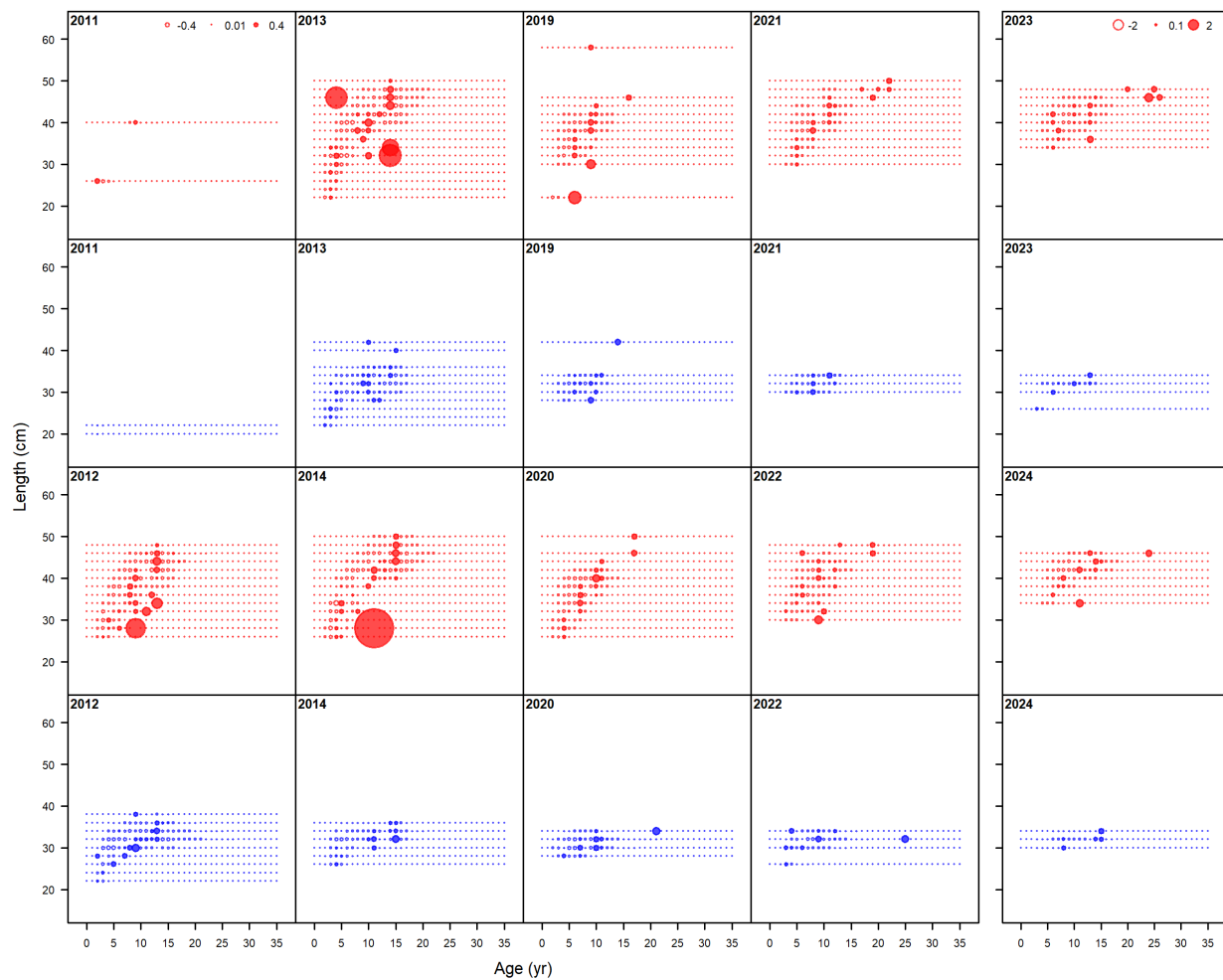
Figure 1E. Pearson residuals for conditional age-at-length data from the California trawl fleet (2011-2024). Length-based selectivity was modeled using the 2D-AR option in Stock Synthesis.
