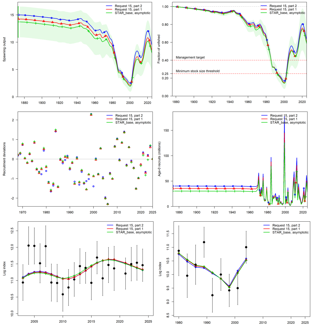
Figure 15C. Spawning output (top left), fraction unfished (top right), recruitment deviations (middle left), age-0 recruits (middle right), log-scale fits to the WCG BTS (bottom left), and log-scale fits to the Triennial survey (bottom right). “Fit” to the Triennial survey index for part 2 is implied with lambda set to zero.
