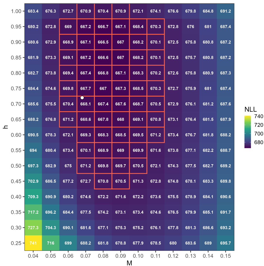
Figure 59: Bivariate profile of natural mortality ( M ) and steepness ( h ) relative with the negative log-likelihood (NLL) value for each model run shown with a white dot indicating the pre-STAR base model values.
