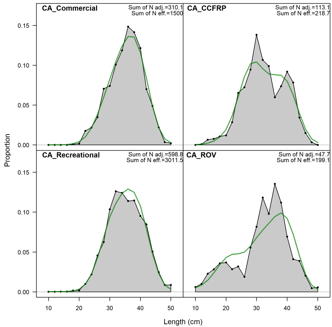
Figure 31: Length composition aggregated across years by fleet with the model with estimated fit to the data by sex (red female, blue male, green unsexed)
