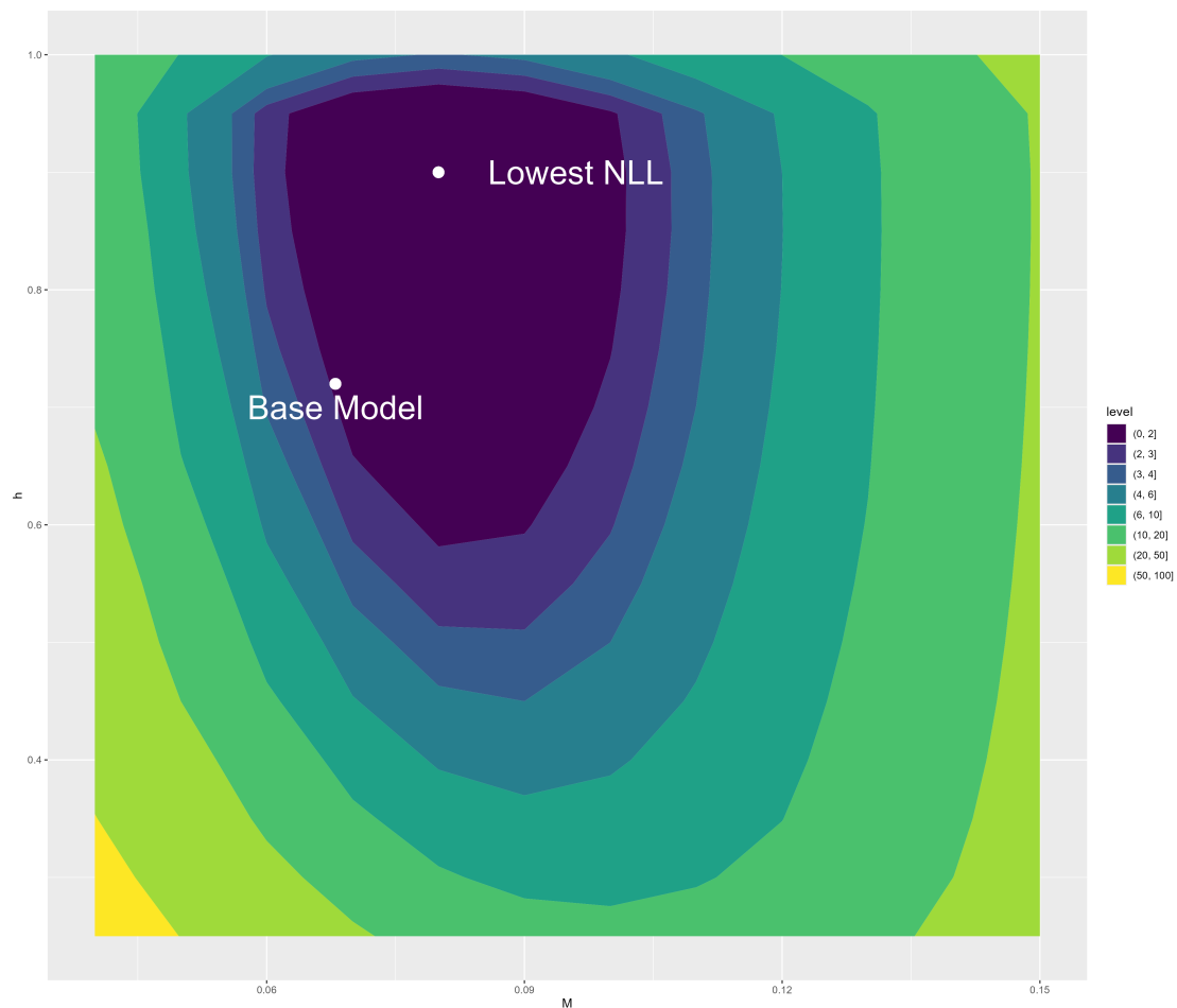
Figure 60: Bivariate profile of natural mortality ( M ) and steepness ( h ) relative to the model with the lowest negative log-likelihood (NLL). The model with the lowest NLL has an approximate value of 0.08 for M and 0.9 for h .
