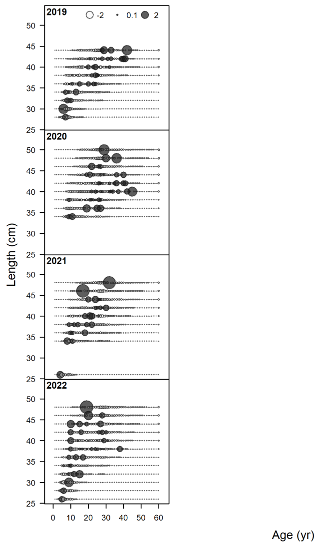
Figure 34: Pearson residuals for the commercial conditional age at length composition.
