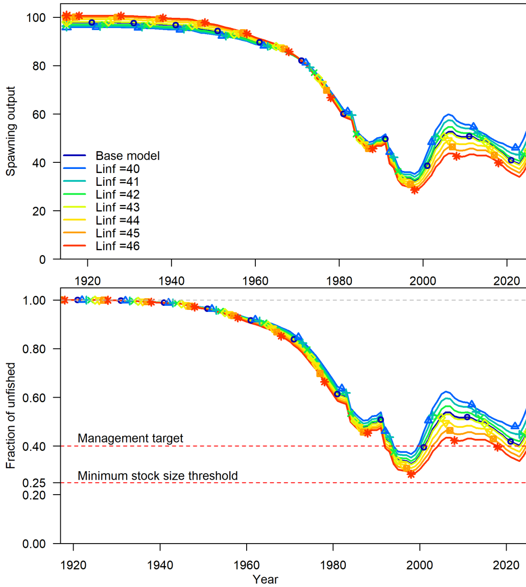
Figure 61: Change in the estimate of spawning output (billions of eggs, top) and spawning output relative to unfished (bottom) across a range of values for asymptotic average length.
