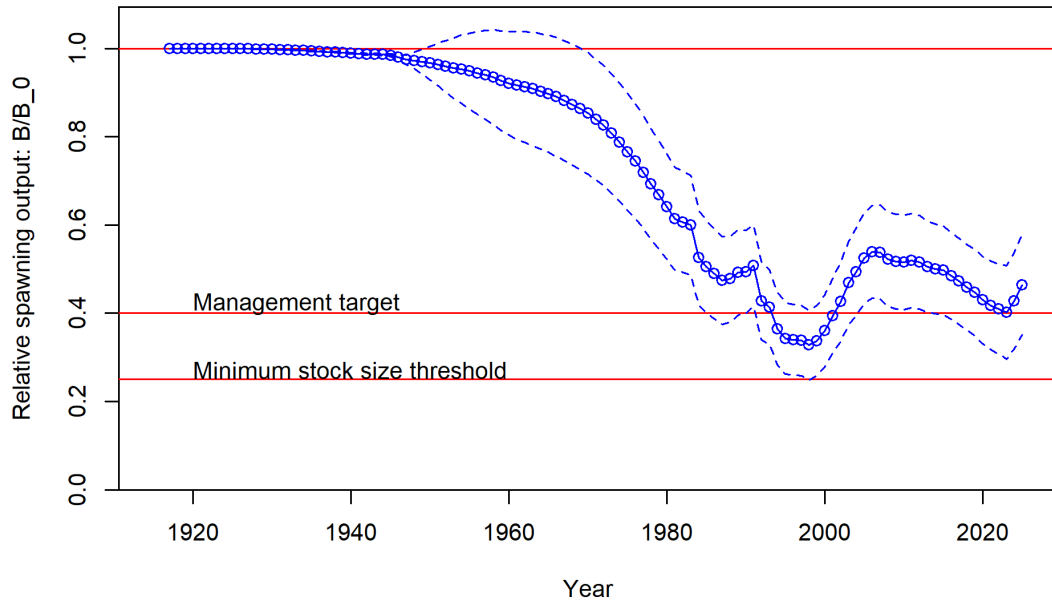
Figure 45: Estimated time series of fraction of unfished spawning output with ~95% asymptotic intervals.
