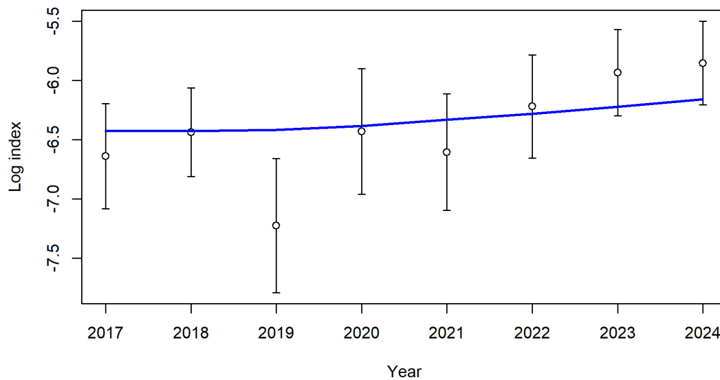
Figure 42: Fit to log index data on log scale for the CCFRP index of abundance. Lines indicate 95% uncertainty interval around index values based on the model assumption of lognormal error.
