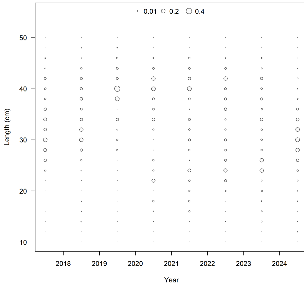
Figure 11: Length composition data for the CCFRP survey where bubbles correspond to the proportional sample size by bin within each year.
