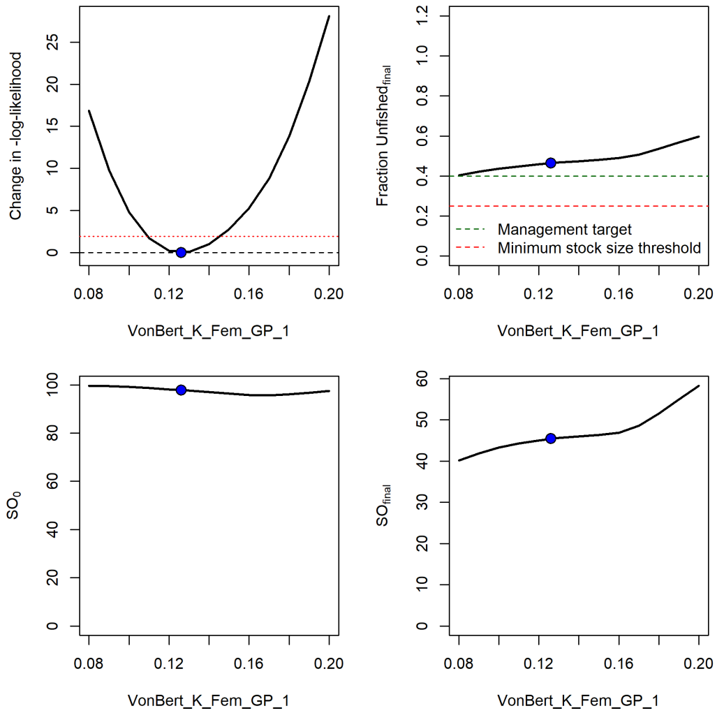
Figure 65: Change in the negative log-likelihood, fraction of unfished spawning output, initial spawning output (in billions of eggs), and final spawning output (in billions of eggs) across a range of values for growth coefficient K.
