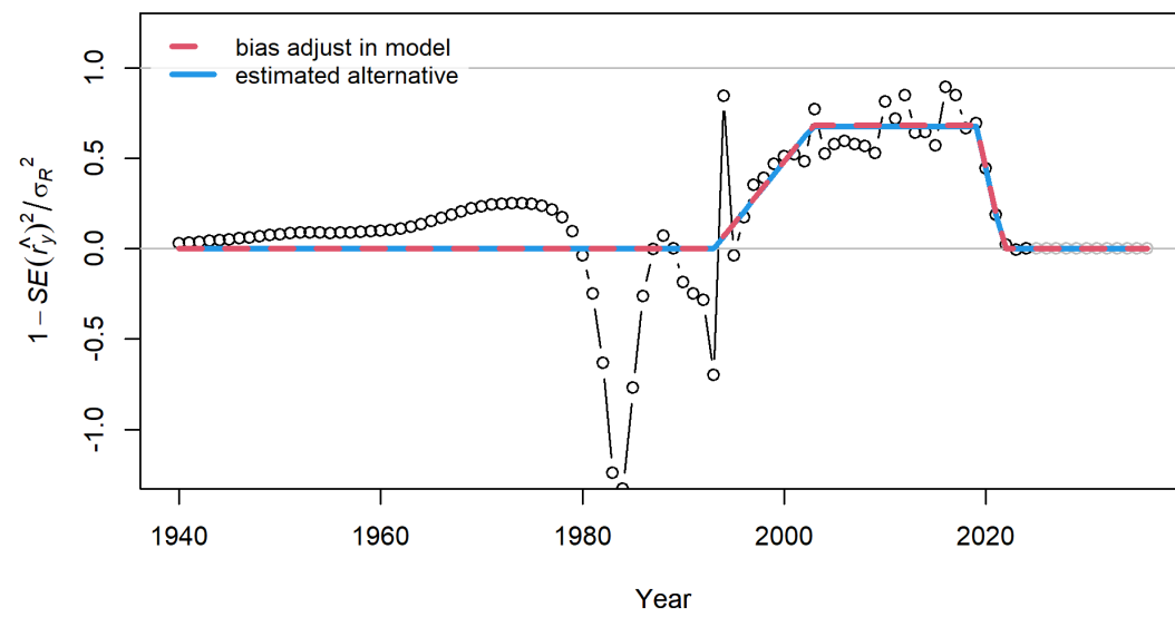
Figure 30: Recruitment bias adjustment applied in the base model. Points are transformed variances. Red line shows current settings for bias adjustment specified in control file. Blue line shows least squares estimate of alternative bias adjustment relationship for recruitment deviations.
