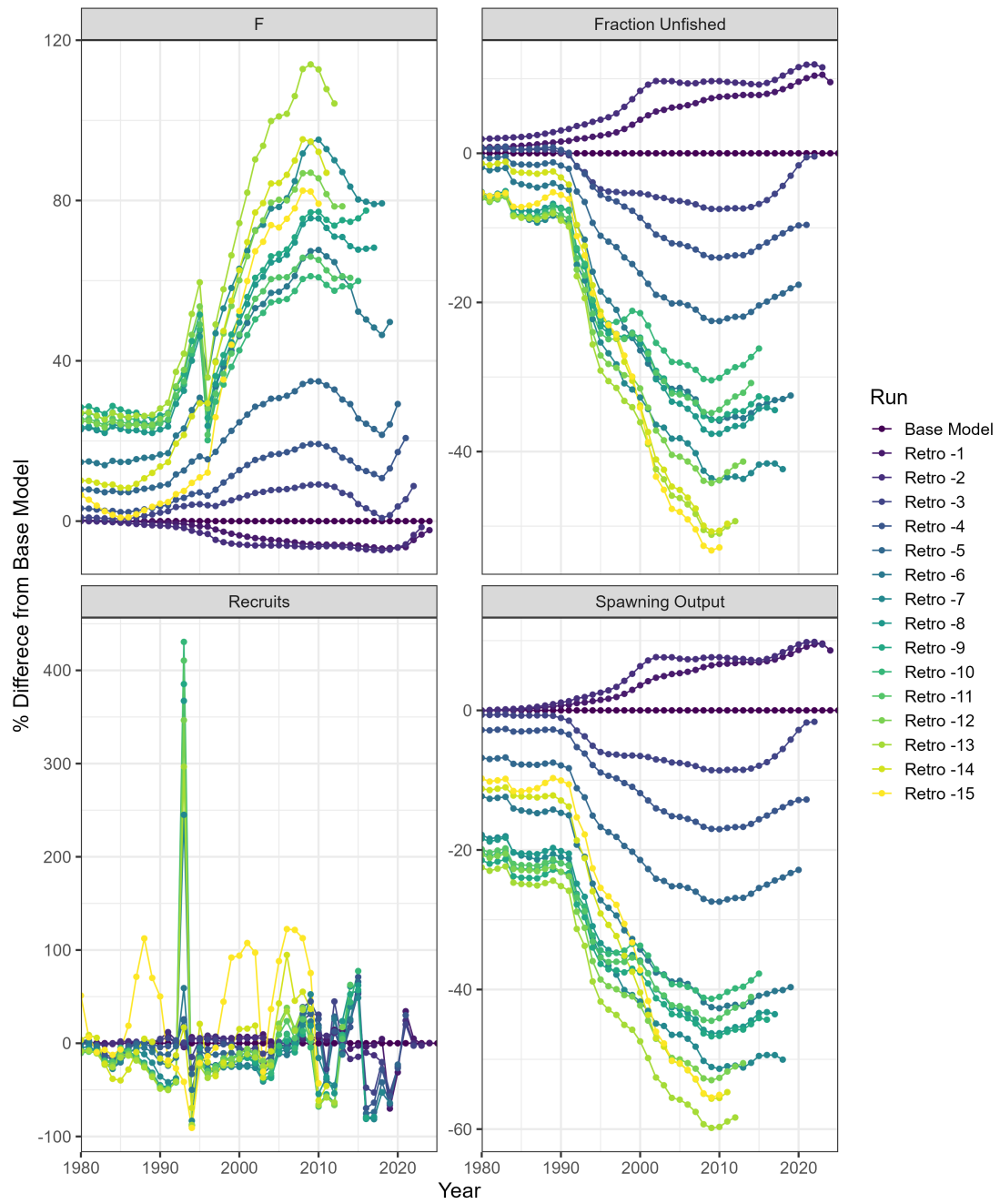
Figure 49: Squid plots of retrospective results relative to the base model for fishing mortality, fraction unfished, recruits, and spawning output (in billions of eggs).
