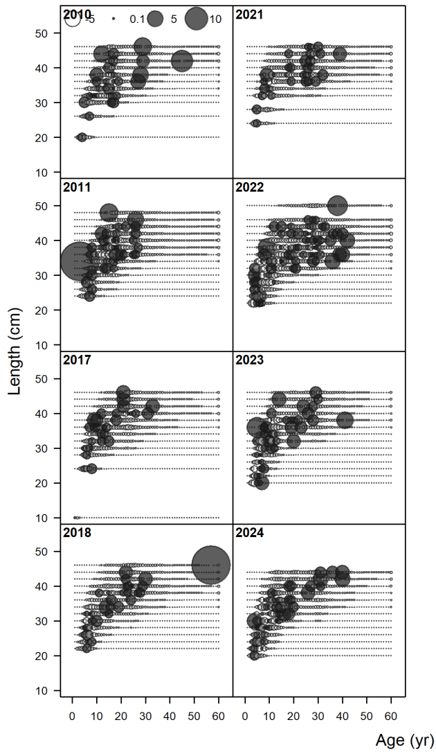
Figure 39: Pearson residuals for the growth fleet conditional age-at-length composition.
