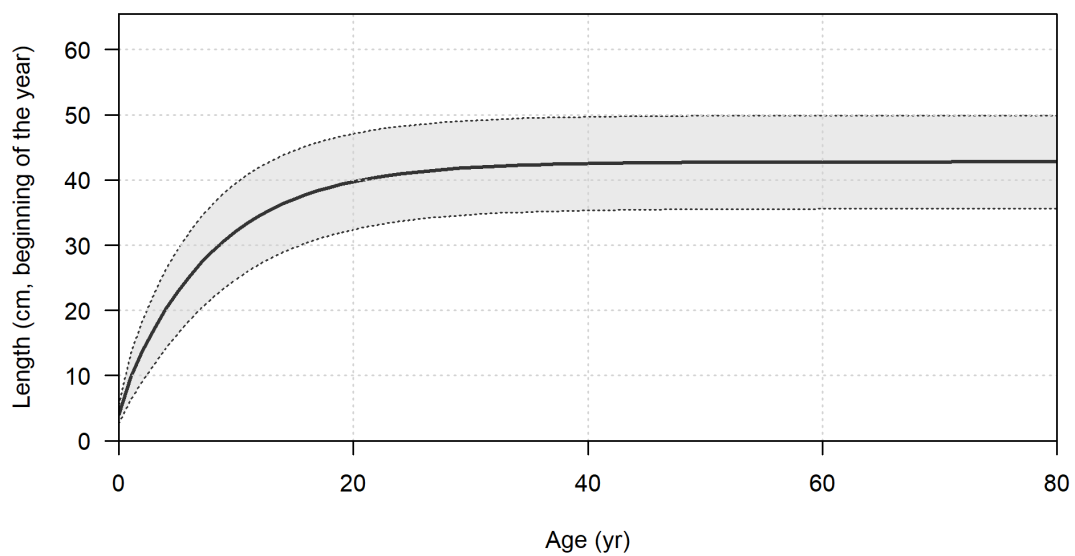
Figure 19: Model estimated length-at-age in the beginning of the year. Shaded area indicates 95 percent distribution of length-at-age around the estimated growth curve.
