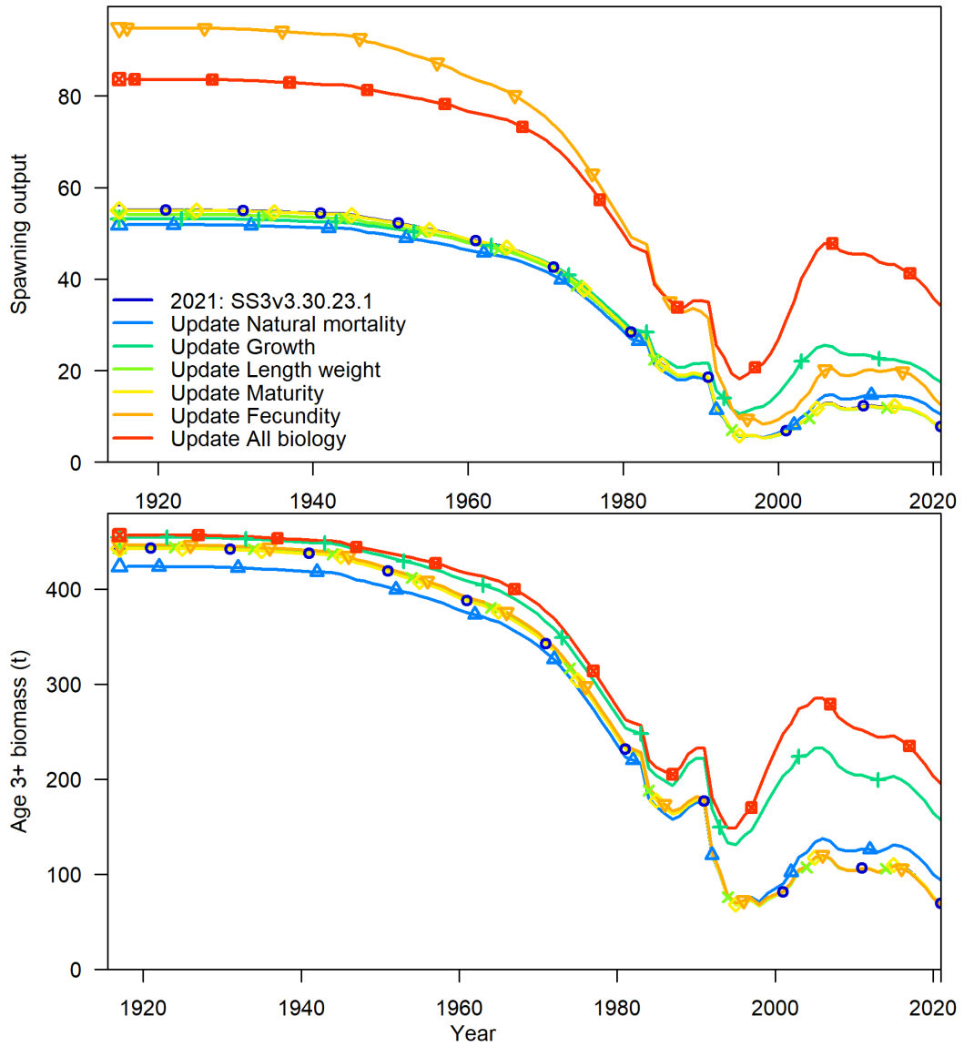
Figure 22: Bridge comparison for biological relationships showing estimated spawning output (billions of eggs, top) and summary biomass (in metric tons, bottom). Each change is tested independently based off the 2021 assessment except the final one (Update All Biology), which combines across all previous changes.
