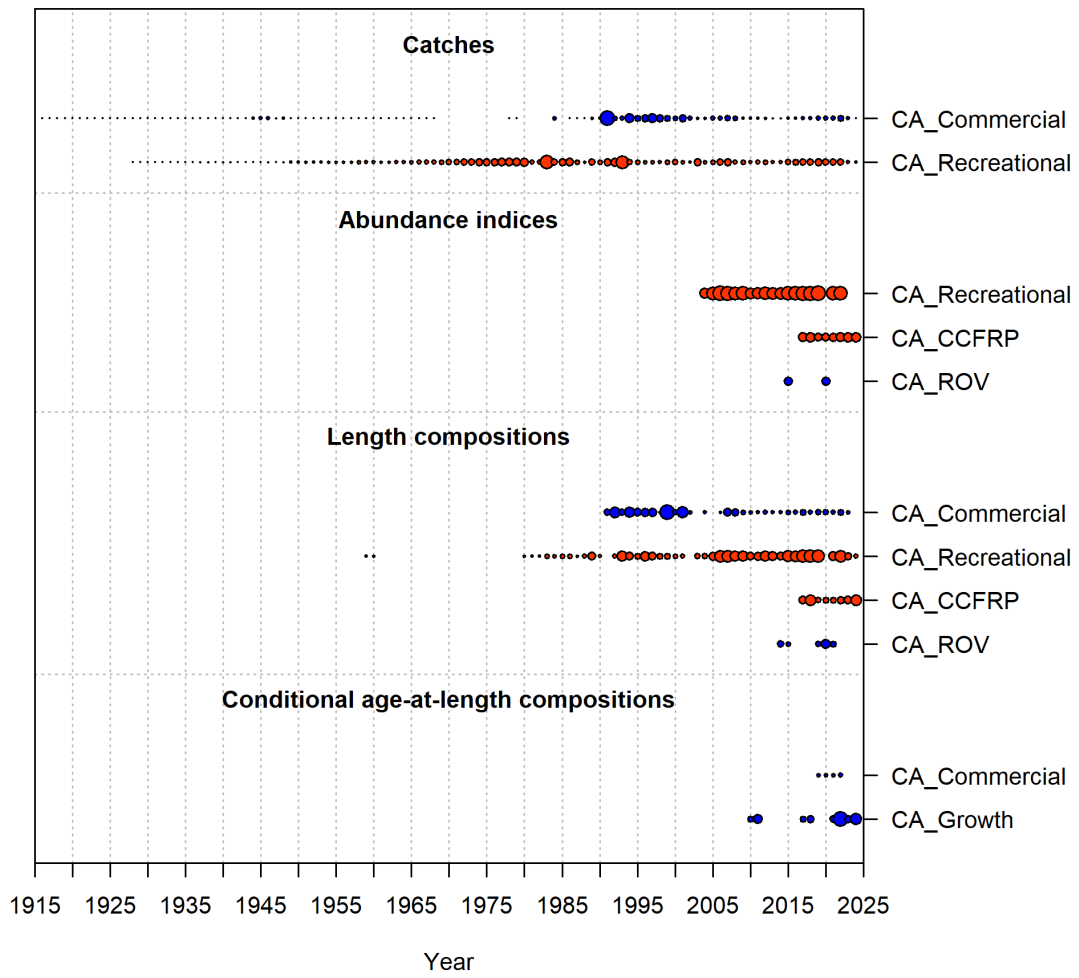
Figure 3: Data available by year for each fleet, where circle area is relative within a data type. Circles are proportional to total catch for catches; to precision for indices, discards, and mean body weight observations; and to total sample size for compositions and mean weight- or length-at-age observations.
