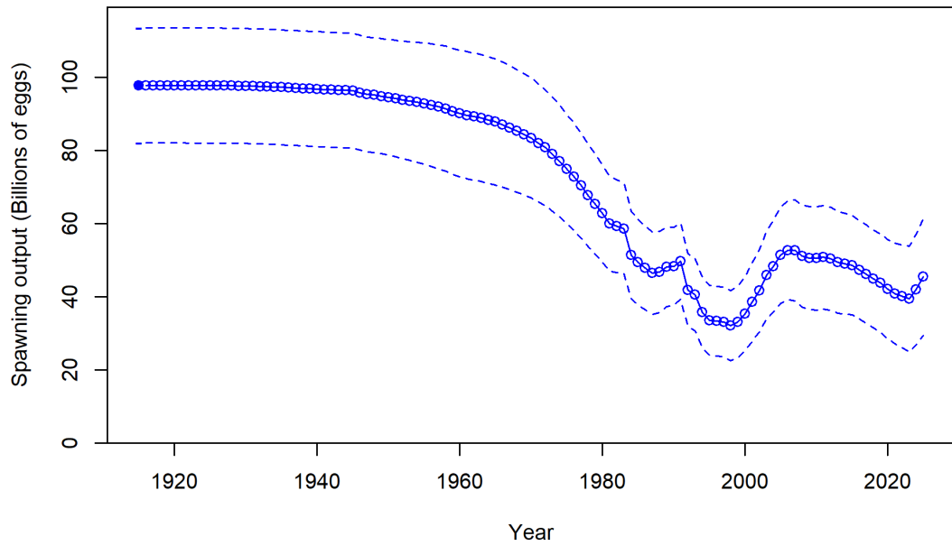
Figure 44: Estimated time series of spawning output in billions of egg with ~95% asymptotic intervals.
