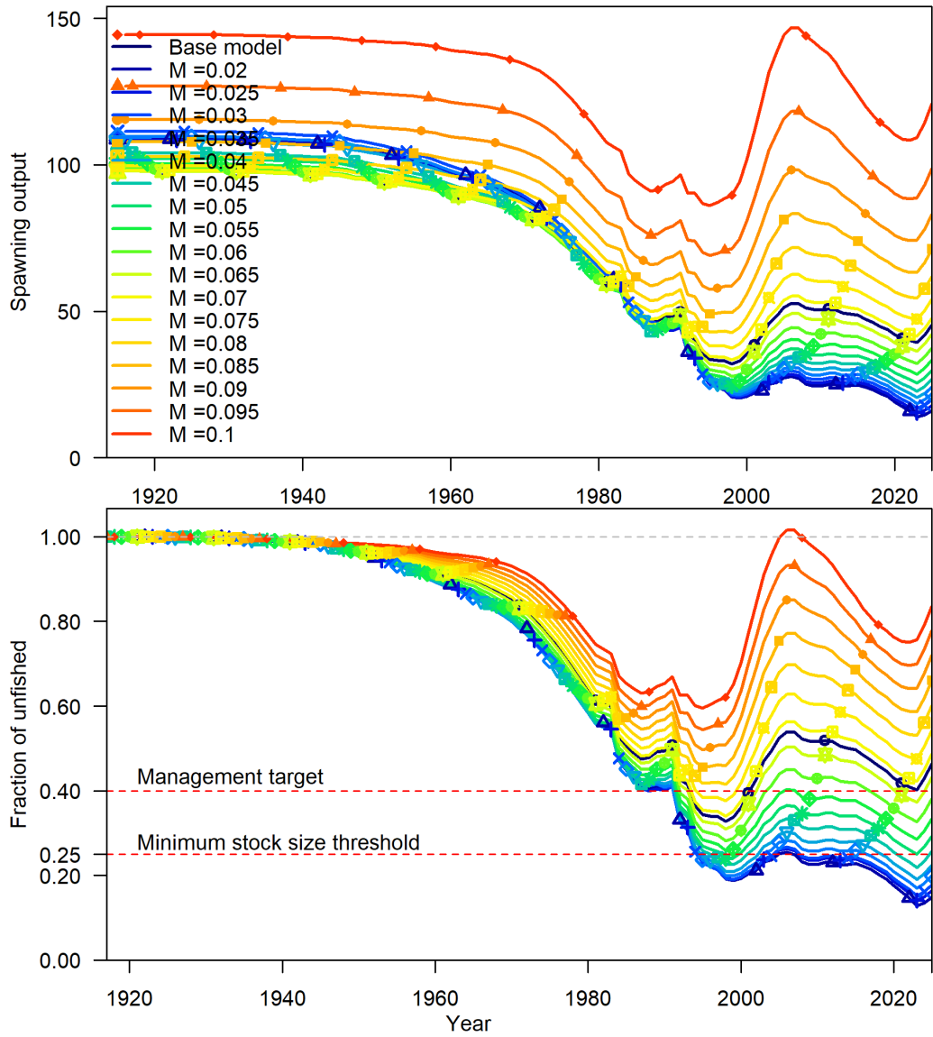
Figure 56: Change in the estimate of spawning output (billions of eggs, top) and spawning output relative to unfished (bottom) across a range of natural mortality values.
