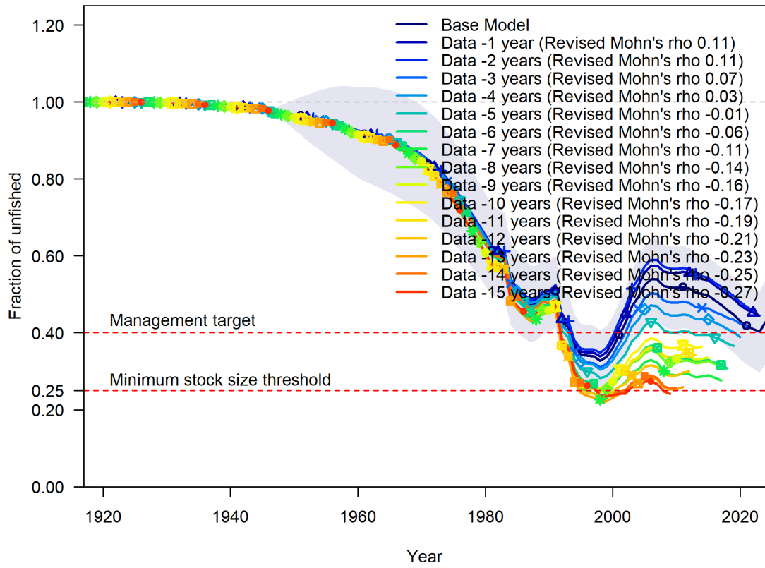
Figure 48: Retrospective results: change in the estimate of the fraction of unfished relative to the start year when the most recent 15 years of data are removed sequentially. The uncertainty shown represents the base model. Mohn's rho values are provided as per year averages.
