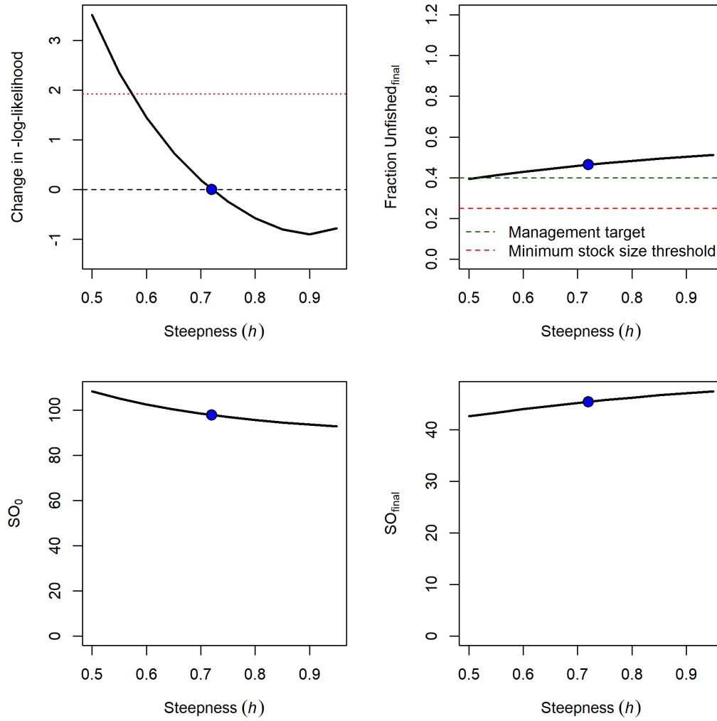
Figure 54: Change in the negative log-likelihood, fraction of unfished spawning output, initial spawning output (in billions of eggs), and final spawning output (in billions of eggs) across a range of steepness values.
