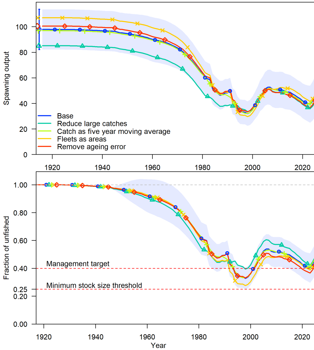
Figure 70: Spawning output (billions of eggs, top), and spawning output relative to unfished (bottom) for data related sensitivities.
