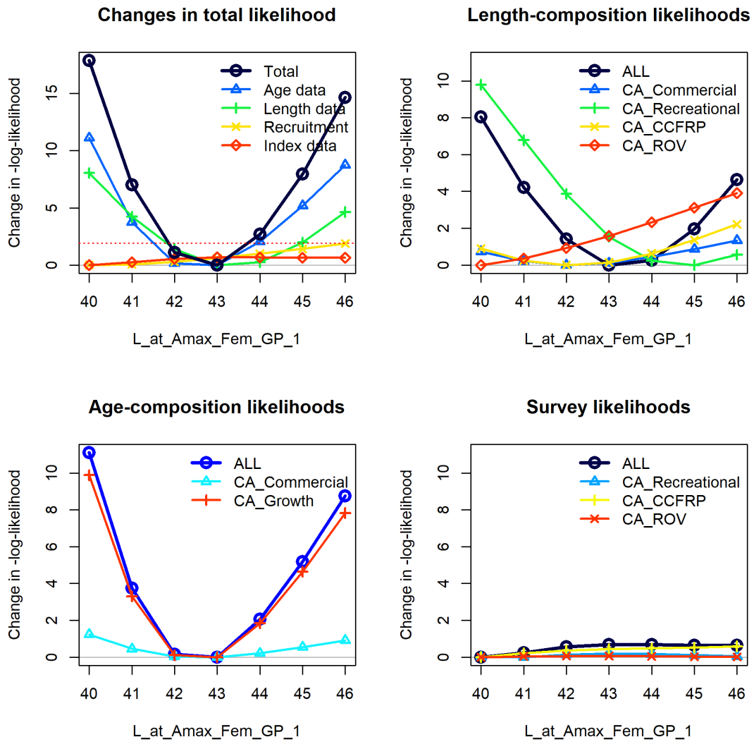
Figure 63: Change in the negative log-likelihood across a range of values for asymptotic average length.
