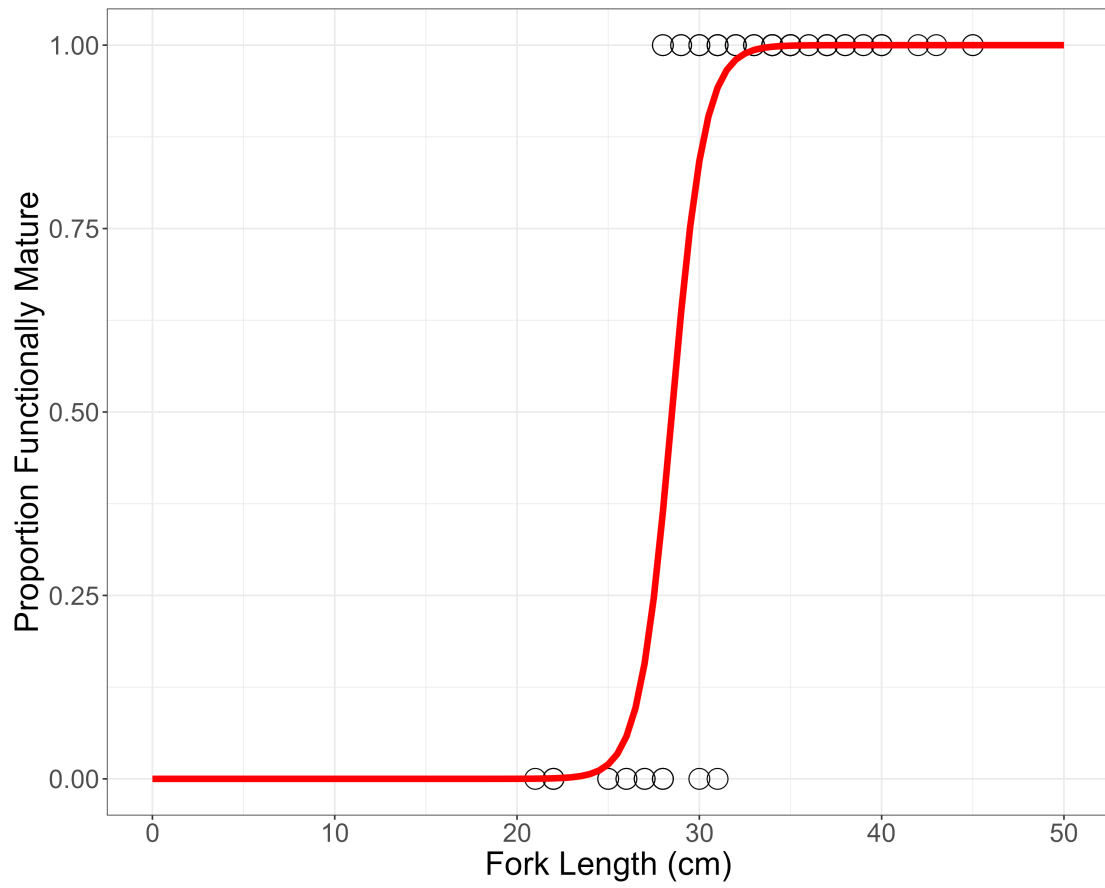
Figure 16: Data and the estimated functional maturity for California quillback rockfish.
