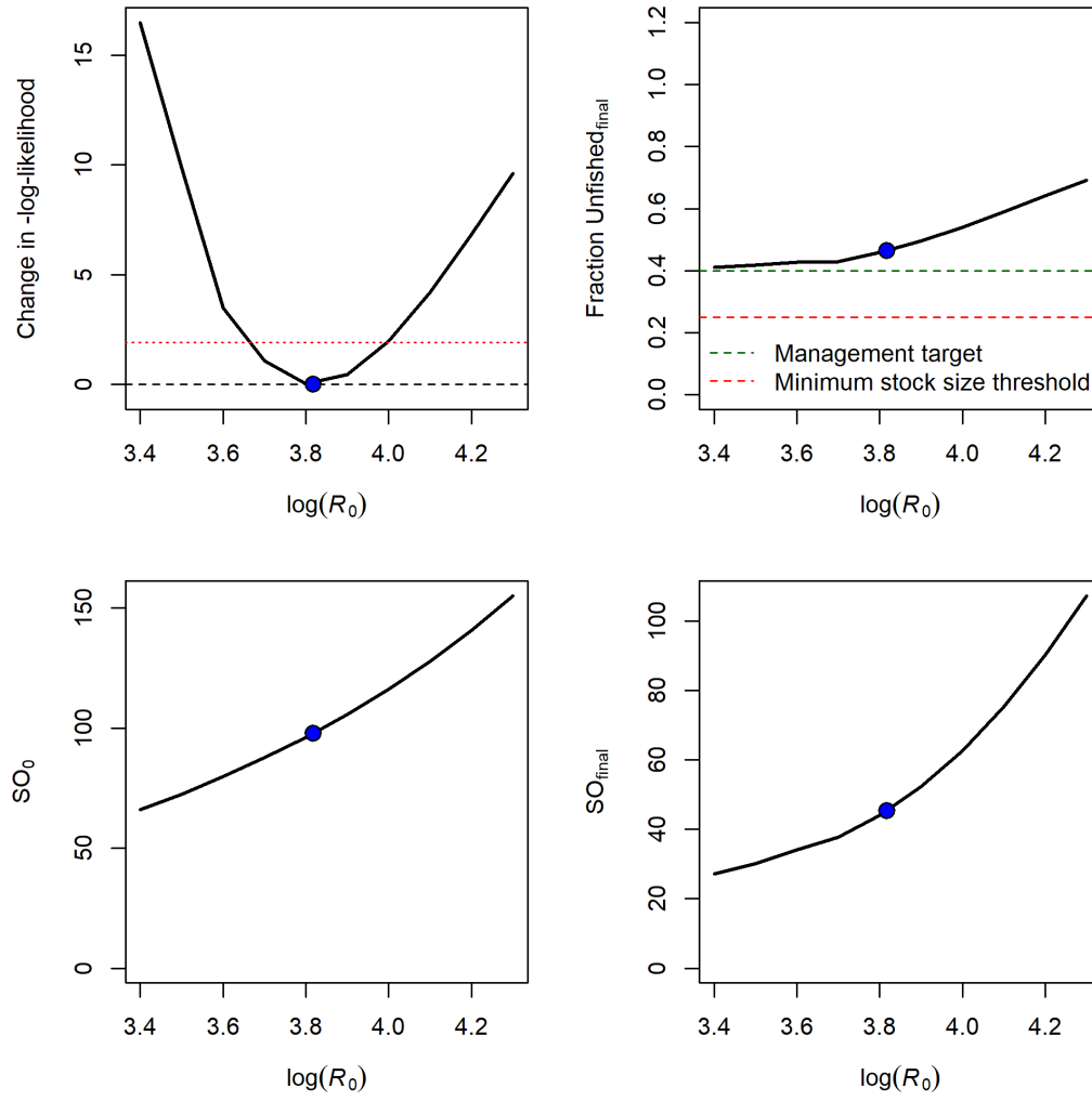
Figure 51: Change in the negative log-likelihood, fraction of unfished spawning output, initial spawning output (in billions of eggs), and final spawning output (in billions of eggs) across a range of \ln(R_0) values.
