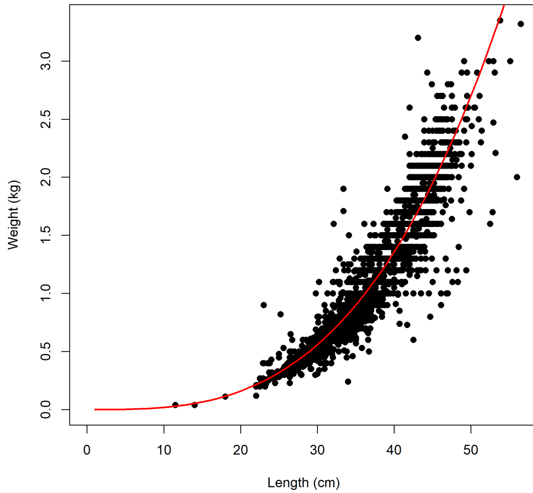
Figure 15: Weight-length relationship with data for California quillback rockfish.
