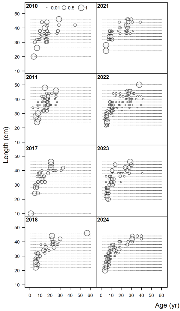
Figure 9: Conditional age-at-length data for the growth fleet where bubbles correspond to the proportional sample size by age for each length bin.
