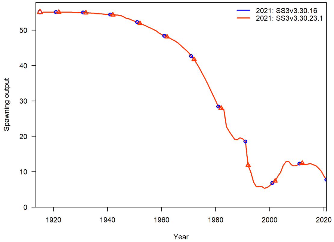
Figure 20: Bridge comparison of estimated spawning output (billions of eggs) of the 2021 assessment with (red line) the newest version of stock synthesis compared to the 2021 version (blue line).
