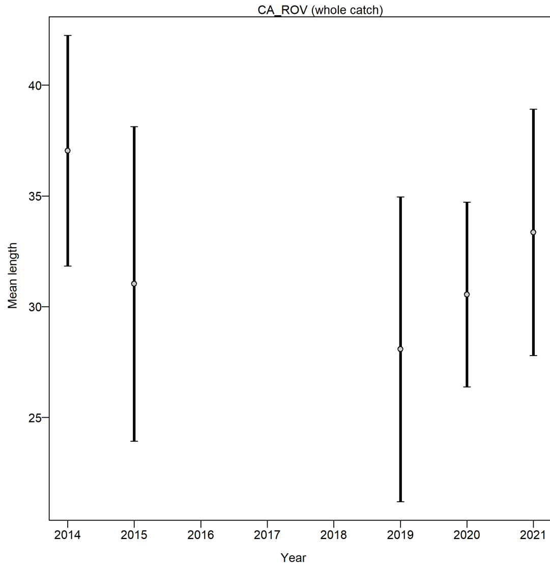
Figure 14: Mean length (cm) for the ROV survey with 95 percent confidence intervals based on current samples sizes.
