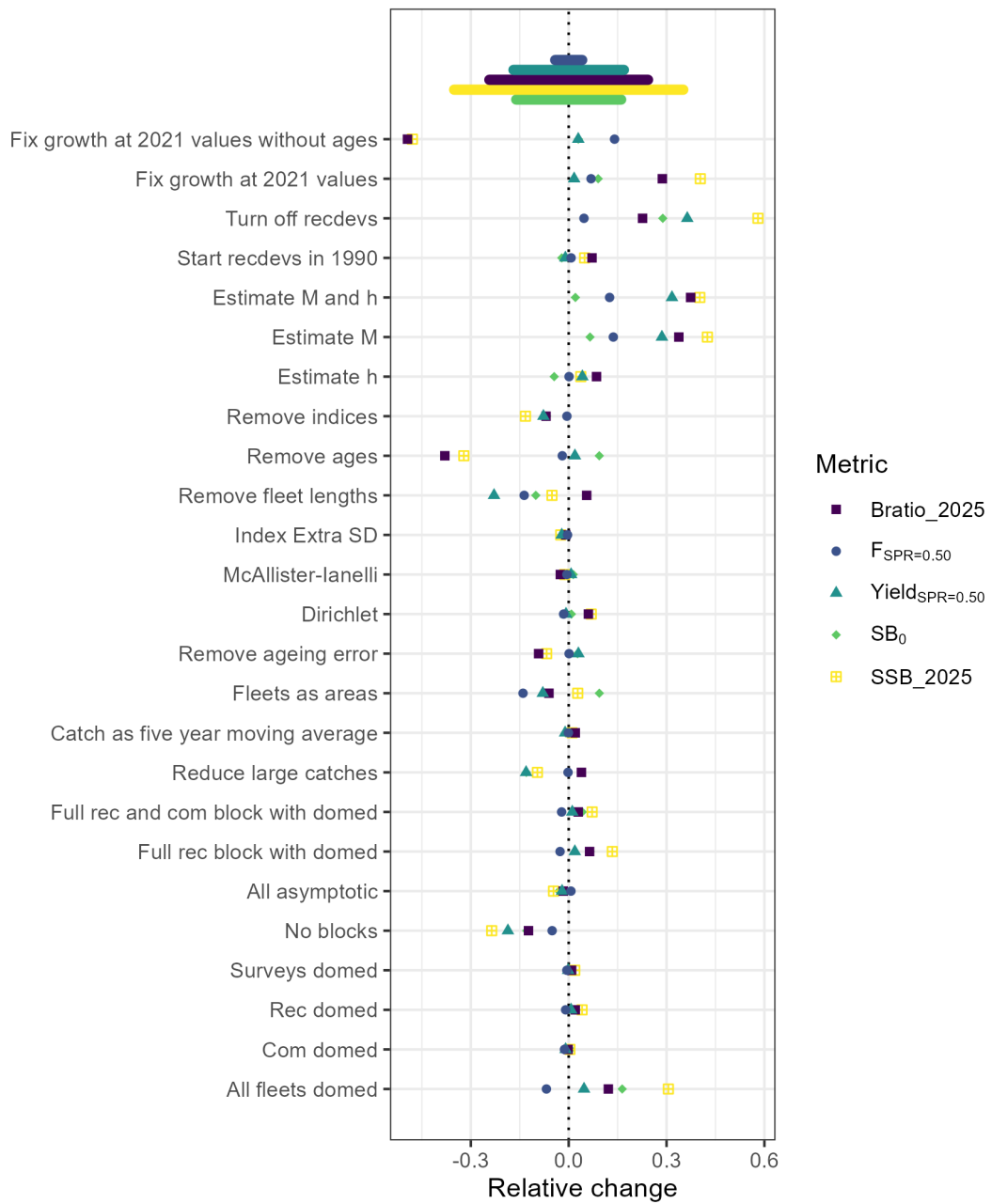
Figure 67: Comparison of various management quantities across all sensitivities. Metrics are terminal year relative spawning output, fishing mortality rate at SPR = 0.5 , yield at SPR = 0.5 , unfished spawning output, and terminal year spawning output. Bars at the top of the figure represent 95% confidence intervals for the metrics in the base model. See legend for which metric each color represents.
