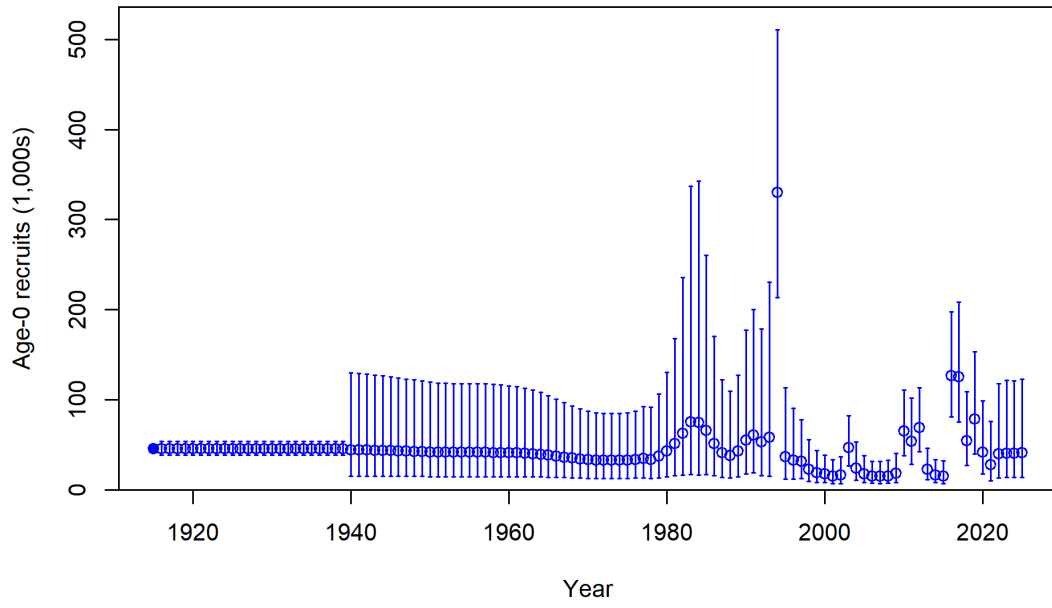
Figure 27: Estimated time series of age-0 recruits with ~95% asymptotic intervals for the base model.
