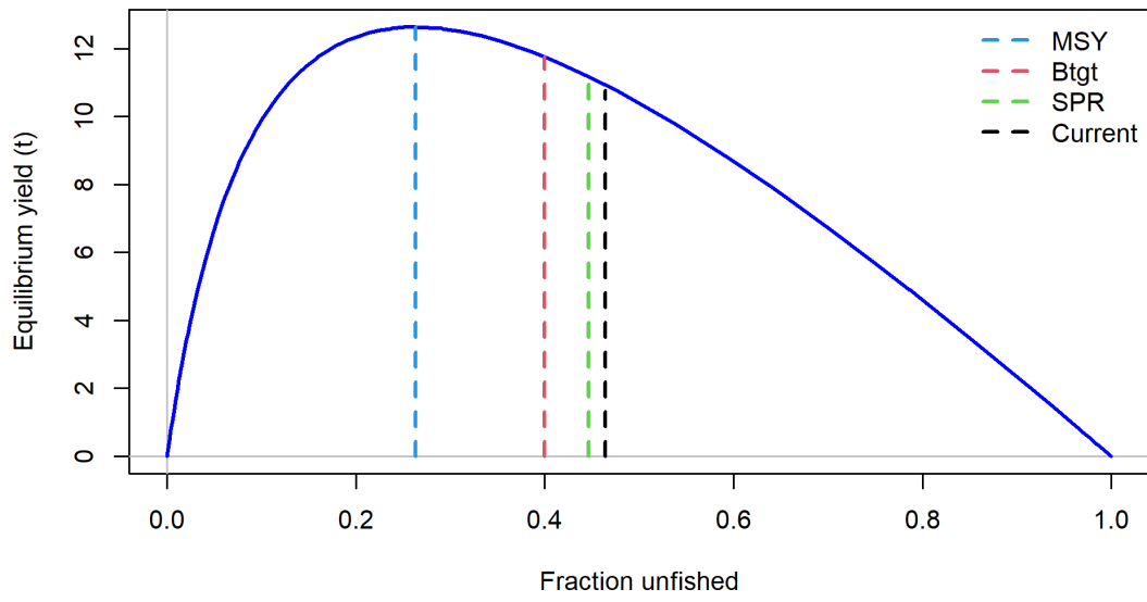
Figure 73: Estimated yield curve with reference points for the base model with yield in mt.
