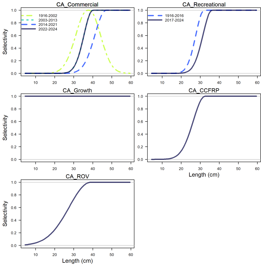
Figure 26: Length-based selectivity showing the time-varying selectivity blocks (in colored lines) for the recreational and commercial fleets as well as the CCFRP, ROV, and growth fleets. Selectivity for the commercial fleet in the 2003–2013 and 2022–2024 blocks are mirrored.
