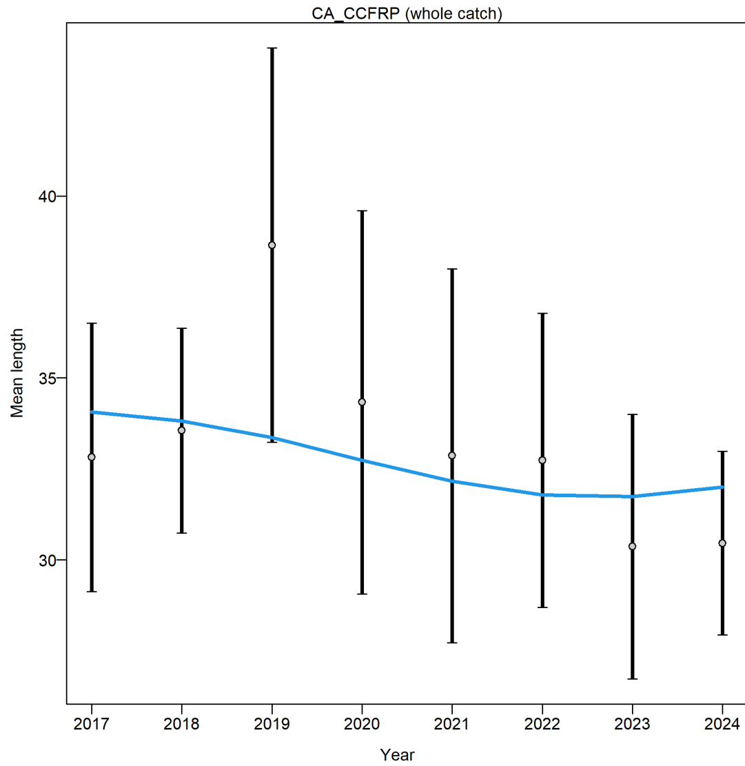
Figure 38: Mean length (cm) for CCFRP with 95% confidence intervals based on adjusted input sample sizes. The blue line is the model expectation.
