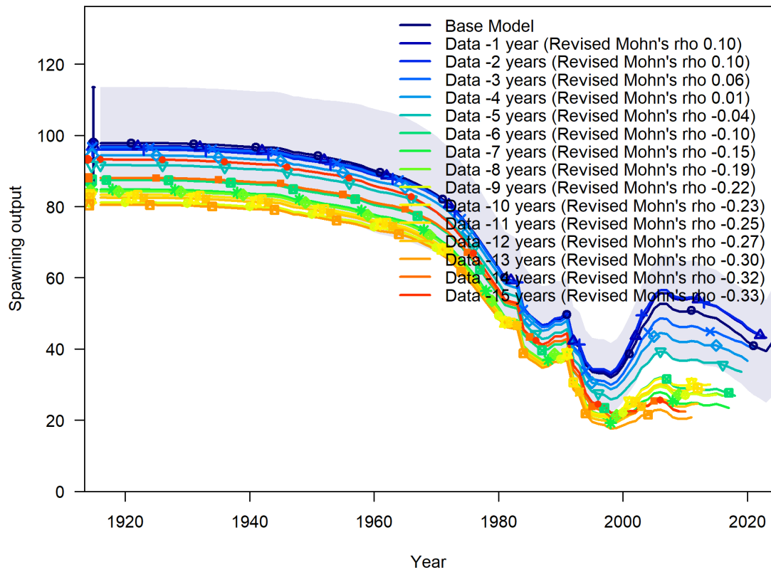
Figure 47: Retrospective results: change in the estimate of spawning output (in billions of eggs) when the most recent 15 years of data area removed sequentially. The uncertainty shown represents the base model. Mohn's rho values are provided as per year averages.
