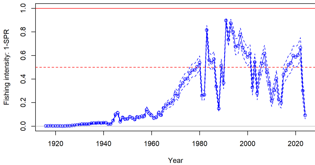
Figure 74: Estimated time series of fishing intensity for the base model.
