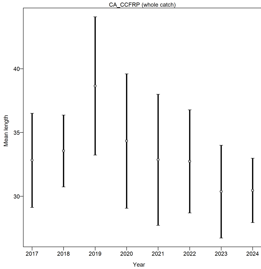
Figure 12: Mean length (cm) for the CCFRP survey with 95% confidence intervals based on current samples sizes.
