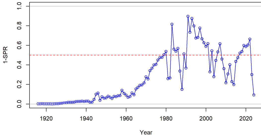
Figure vi: Time series of 1-SPR (spawning potential ratio). The horizontal line is at 1-SPR target: 1 - 0.5 = 0.5
