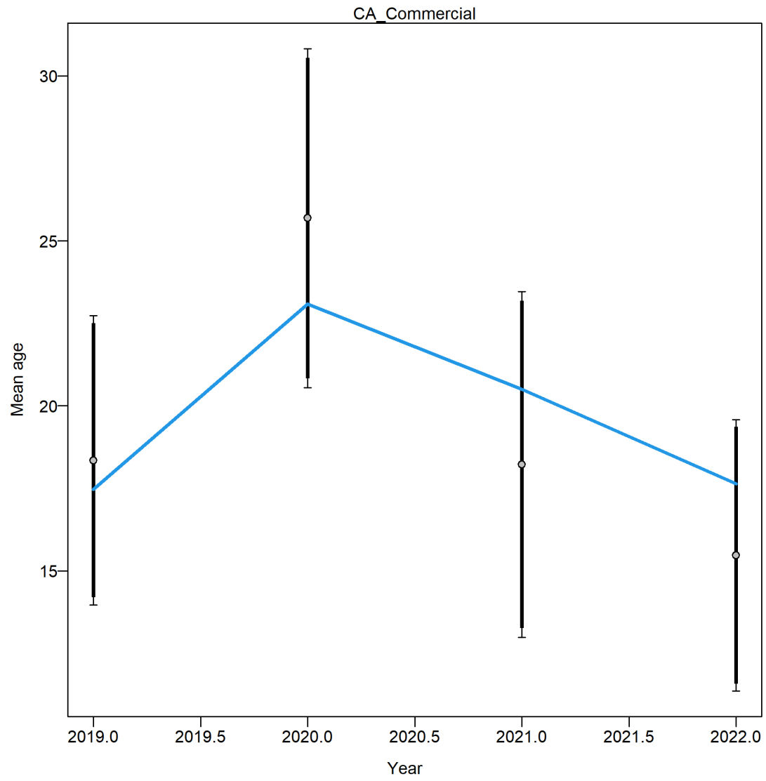
Figure 35: Mean age from conditional data (aggregated across length bins) for the commercial fleet with 95% confidence intervals based on current samples sizes.
