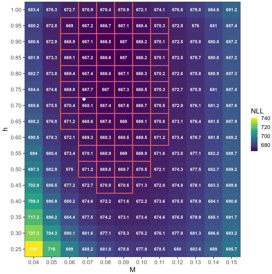
Figure 59: Bivariate profile of natural mortality (M) and steepness (h) relative with the negative log-likelihood (NLL) value for each model run shown with a white dot indicating the pre-STAR base model values.
