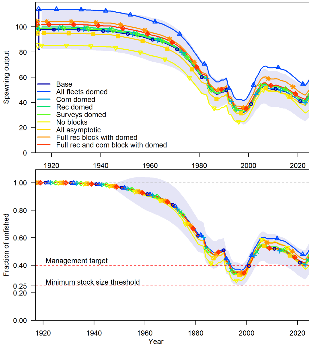
Figure 71: Spawning output (billions of eggs, top), and spawning output relative to unfished (bottom) for selectivity related sensitivities.
