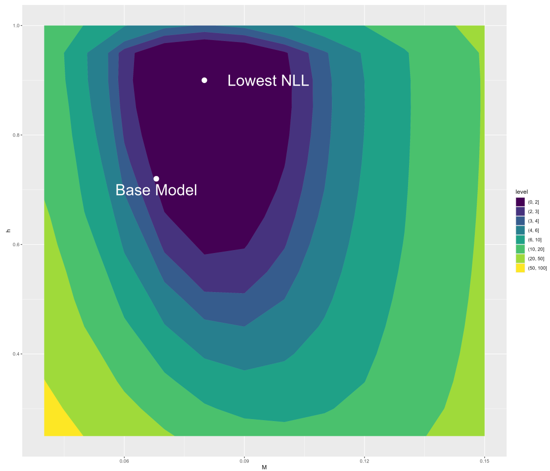
Figure 60: Bivariate profile of natural mortality (M) and steepness (h) relative to the model with the lowest negative log-likelihood (NLL). The model with the lowest NLL has an approximate value of 0.08 for M and 0.9 for h.
