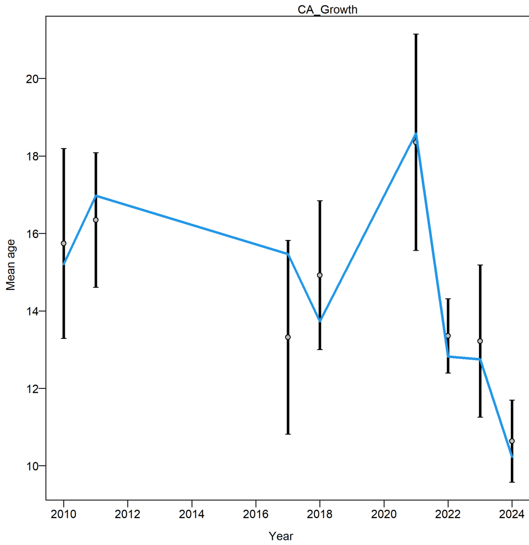
Figure 40: Mean age from conditional age-at-length data (aggregated across length bins) for the growth fleet with 95% confidence intervals based on current samples sizes.
