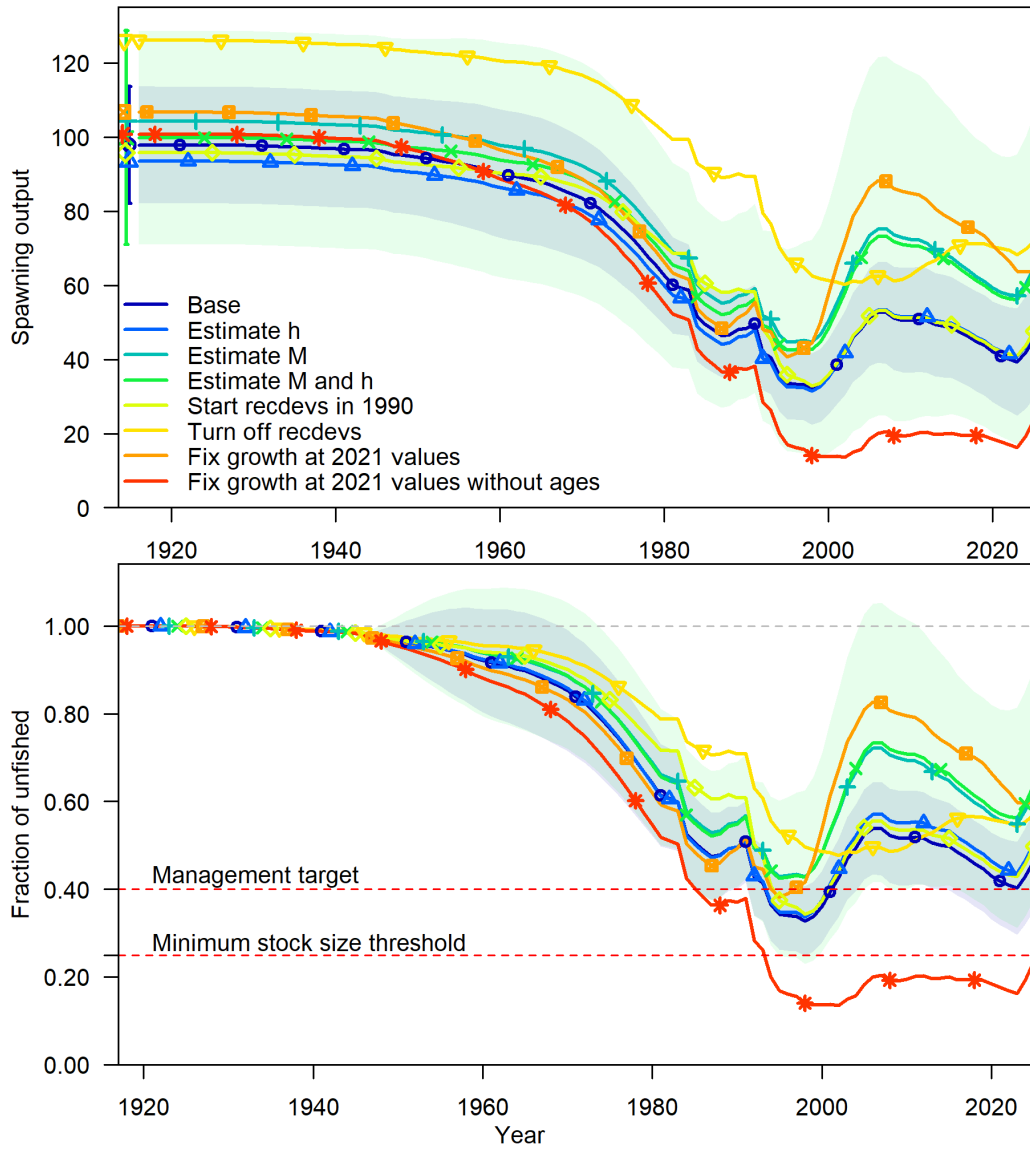
Figure 68: Spawning output (billions of eggs, top), and spawning output relative to unfished (bottom) for productivity related sensitivities.
