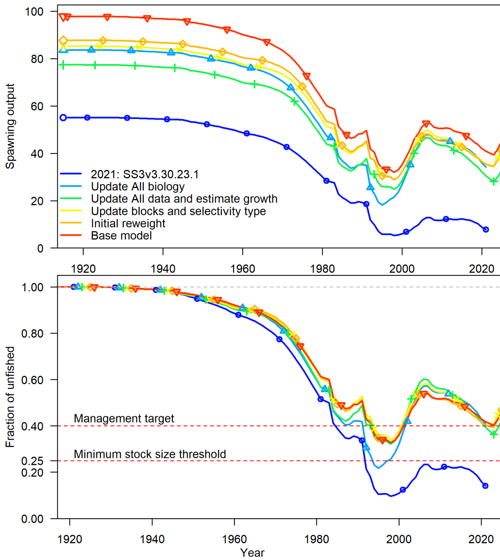
Figure 24: Bridge comparisons showing estimated spawning output (billions of eggs, top) and spawning output relative to unfished (bottom) when updating selectivity and reapplying data weighting procedures. Each step reflects sequential changes leading up to the final base model, which includes additional minor changes as described in the text.
