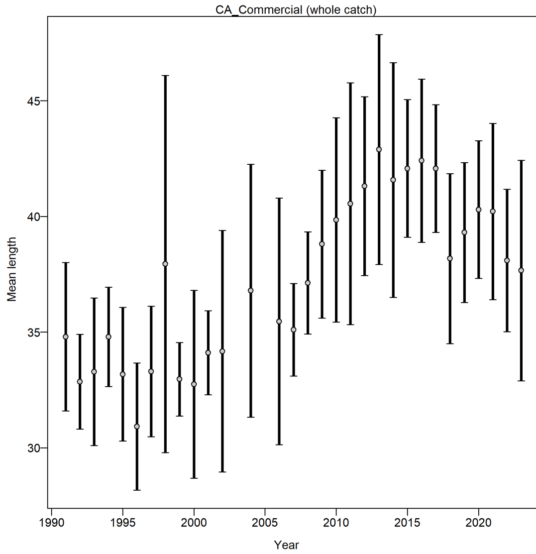
Figure 5: Mean length (cm) for the commercial fleet with 95 percent confidence intervals based on current samples sizes.
