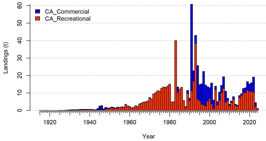
Figure 2: Total removals for quillback rockfish in California from 1916-2024 for the commercial (blue bars; CA_Commercial) and recreational (red bars; CA_Recreational) fleets. The y-axis units are metric tons.
