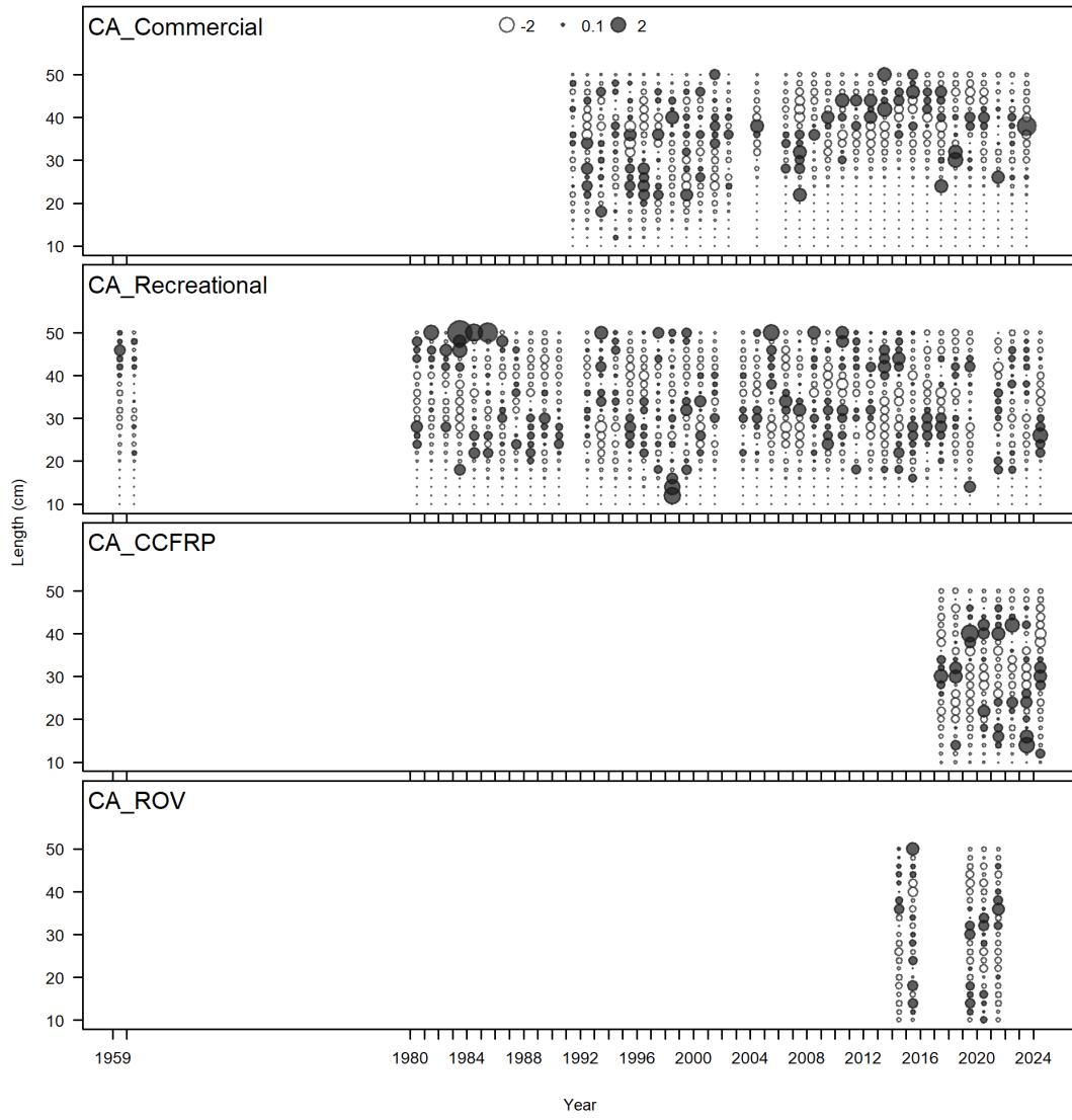
Figure 32: Pearson residuals for fit to length composition data for all fleets (red female, blue male, grey unsexed). Closed bubbles are positive residuals (observed > expected) and open bubbles are negative residuals (observed < expected).
