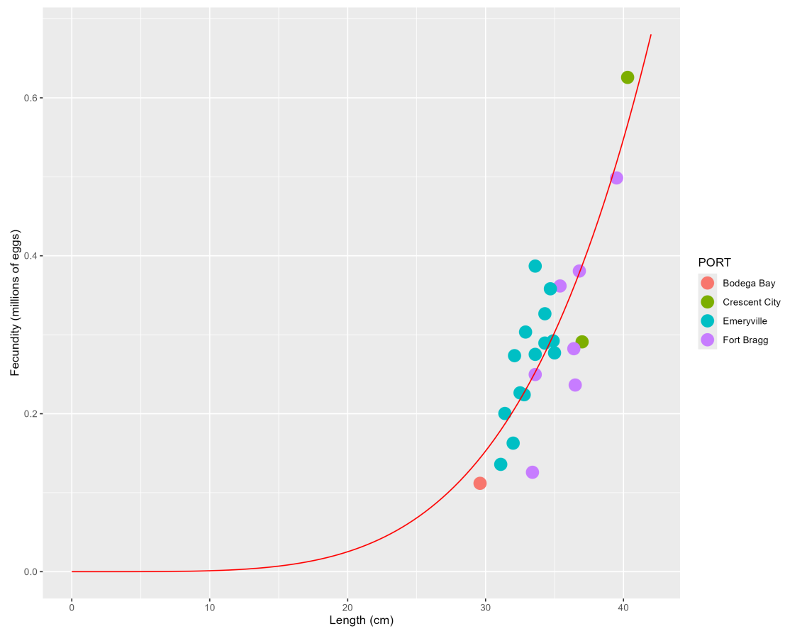
Figure 17: Fecundity estimated from samples collected by the SWFSC from across the range of California quillback rockfish.
