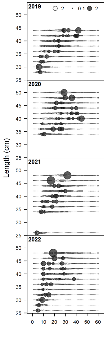
Figure 34: Pearson residuals for the commercial conditional age at length composition.
