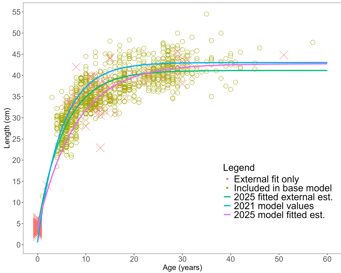
Figure 18: Available length-at-age data for the 2025 stock assessment. Growth curves are provided based on the external estimate of the data (open circles and Xs), and from the internally estimated values within the base model (open circles only). The fixed values from the 2021 assessment are also provided for comparison.
