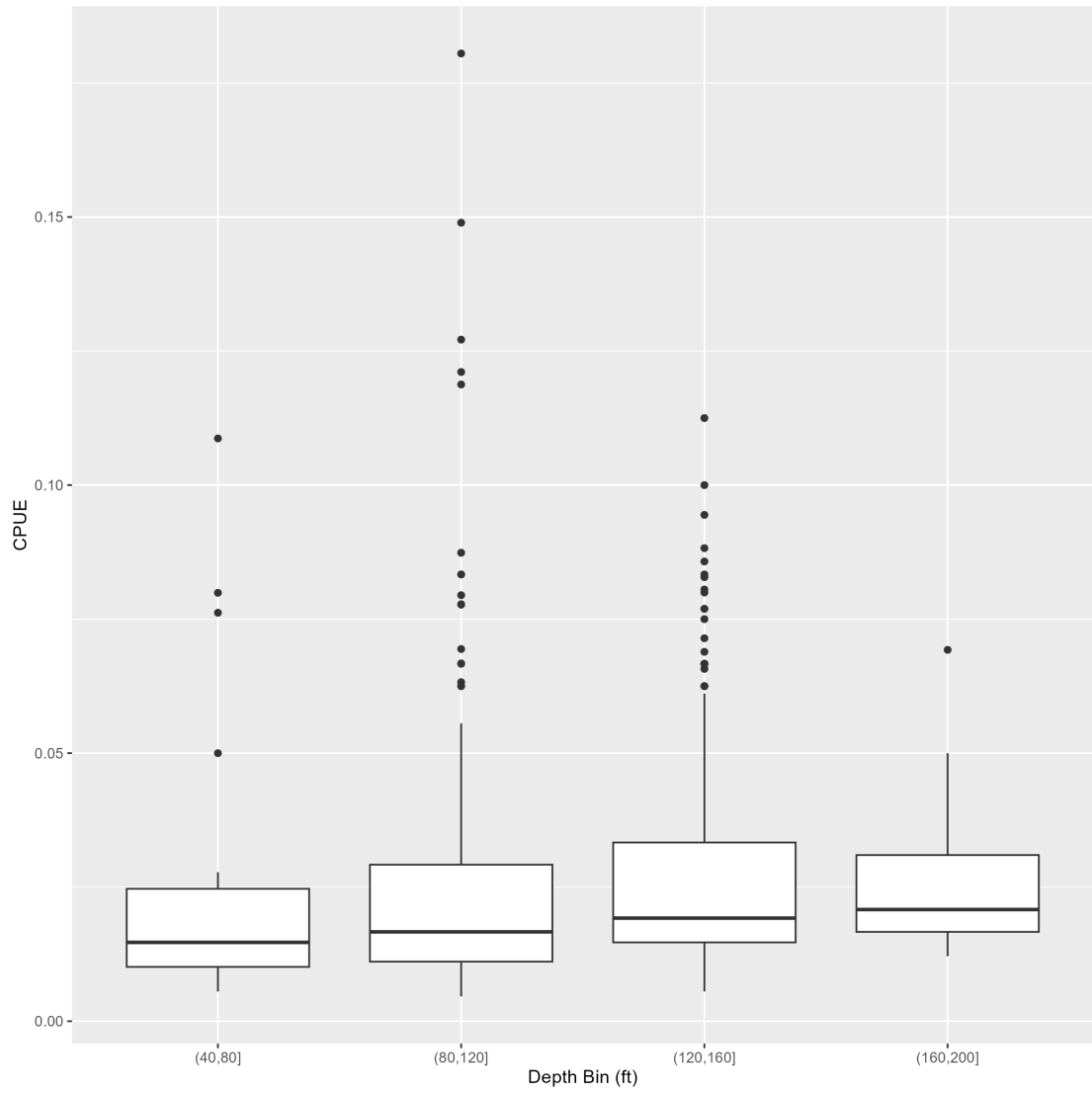
Figure A-9: CPUE across 40 foot depth bins.
