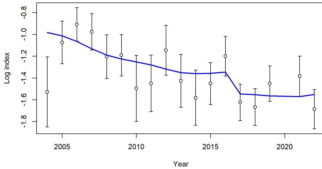
Figure 41: Fit to log index data on log scale for the CRFS dockside private/rental index of abundance. Lines indicate 95% uncertainty interval around index values based on the model assumption of lognormal error.
