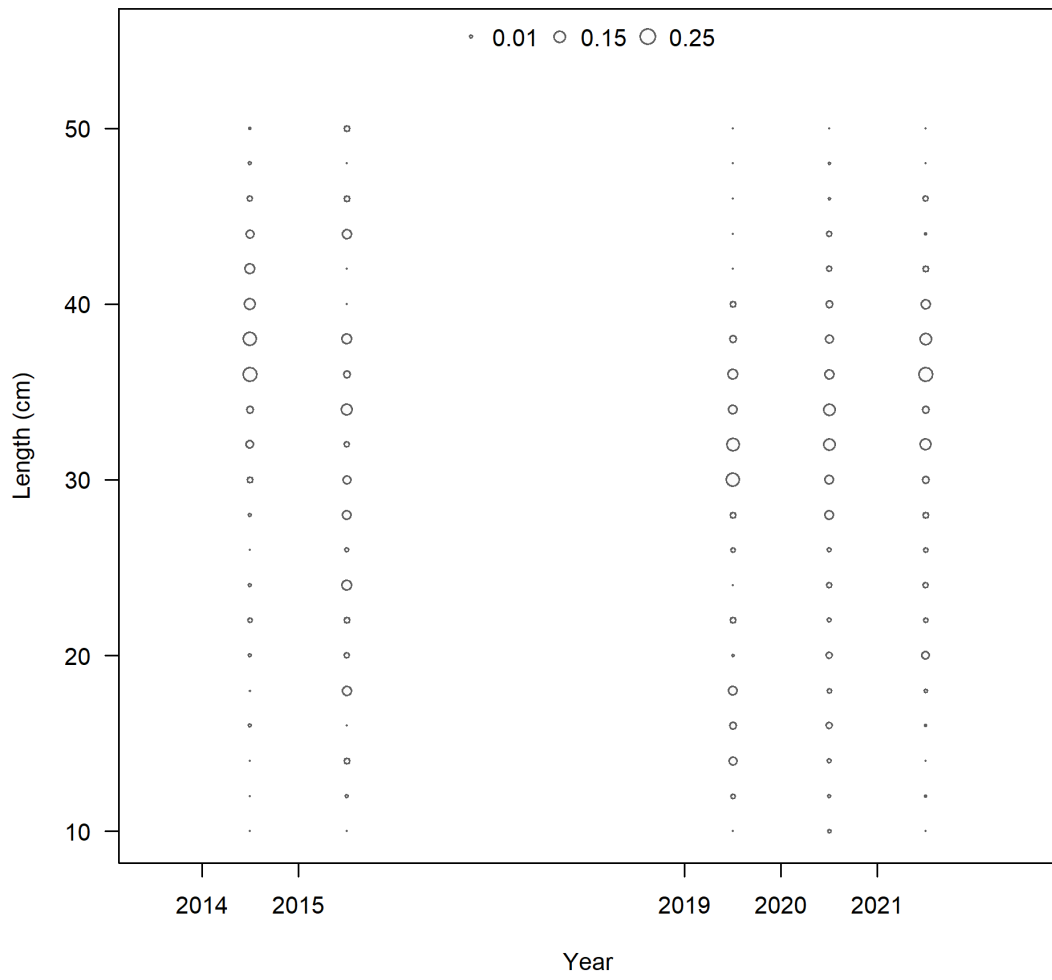
Figure 13: Length composition data for the ROV survey where bubbles correspond to the proportional sample size by bin within each year.
