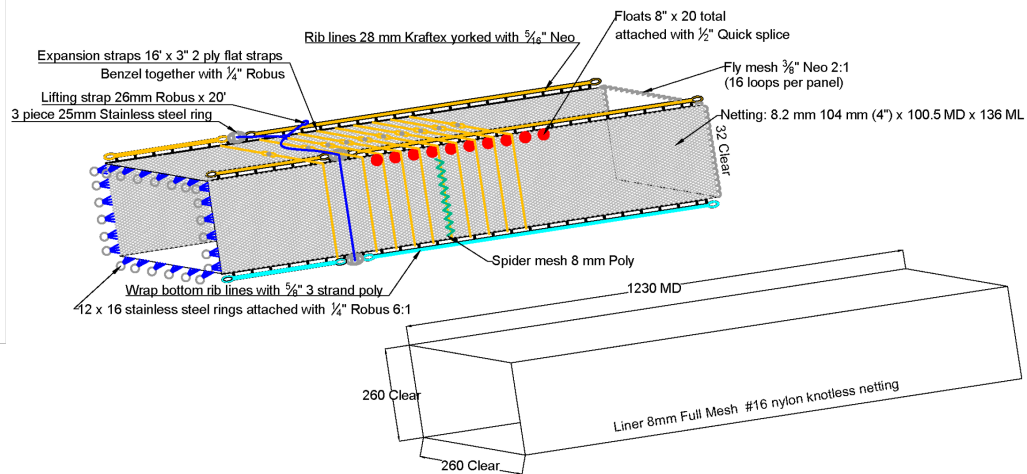
Figure 7: Schematics of the Multifunction Trawl Net System a) rigging and b) cod-end.
