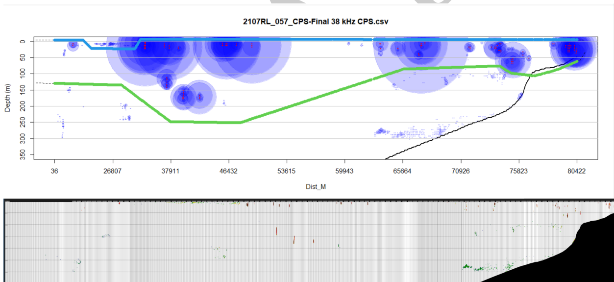
Figure 11: Echoes from fish with swimbladders (blue points, scaled by backscatter intensity) along an example acoustic transect (top) and the corresponding echogram image (bottom). In this example, the upper (blue) and lower lines (green) indicate boundaries within which echoes were retained. Where the lower boundary was deeper than the seabed (black line), echoes above the seabed were retained. Echoes from deep, bottom-dwelling schools of non-CPS fishes with swimbladders, and from diffuse scatterers near the surface were excluded.
